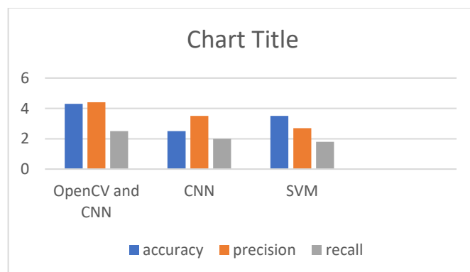
Figure 2 Accuracy Graph
