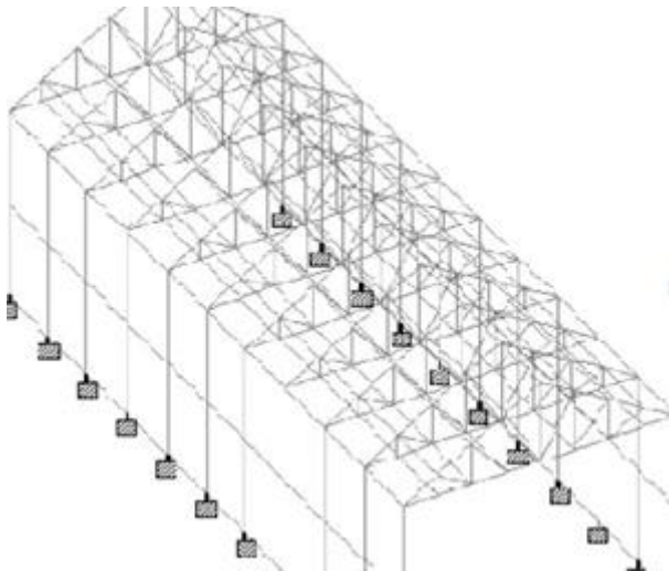
Fig: Structure of roof truss from STAD Pro [ Refer from STAAD Pro]
