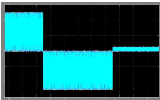
Fig.3.6. 3 Phase currents.
